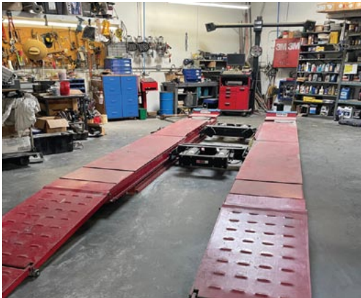
Hunter WA240 alignment analyzer with Hawkeye sensors and 12,000lb capacity scissor lift alignment rack
