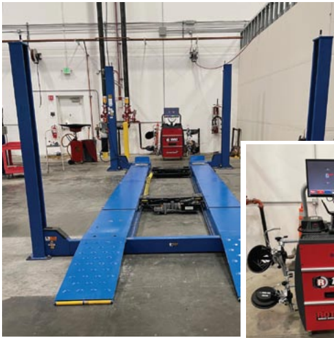
Rotary R 1080 alignment analyzer (Mfg. 2020) with Rotary 14K capacity 4-post alignment rack (Mfg. 2022)
